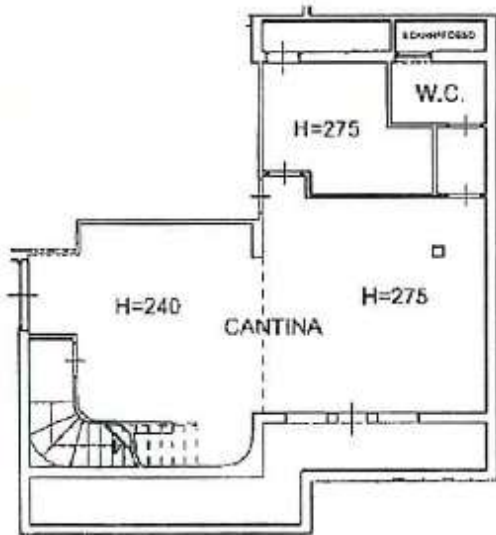
PIANO INTERRATO
